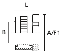
HelaGuard fitting, plain hole connector
